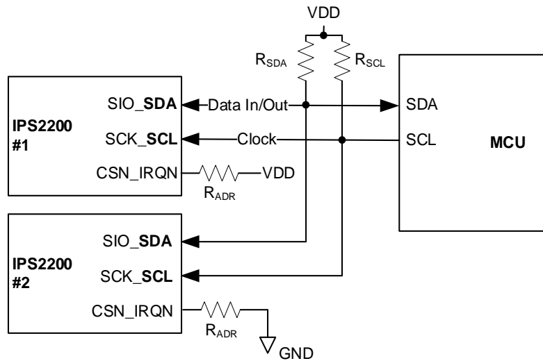
Figure 20. I2C Interface with Address Select
