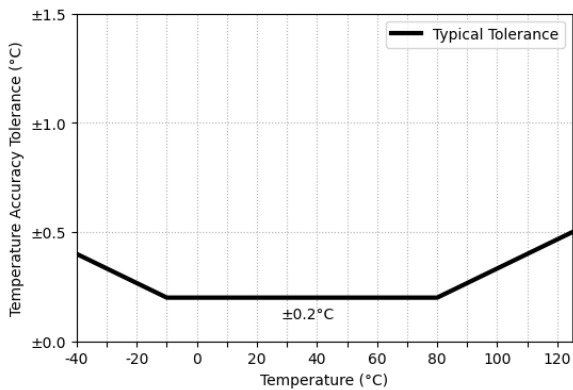
Figure 8. HS3xx1-ML1 Temperature Sensor Accuracy Tolerance
