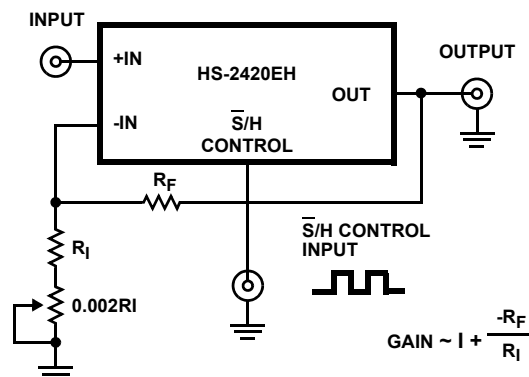
FIGURE 19. NONINVERTING CONFIGURATION WITH GAIN ADJUST
