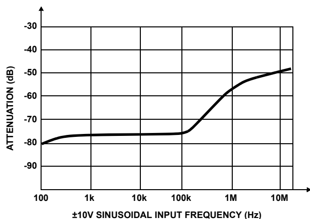
FIGURE 14. HOLD MODE FEEDTHROUGH ATTENUATION CH = 1000\text{pF}
