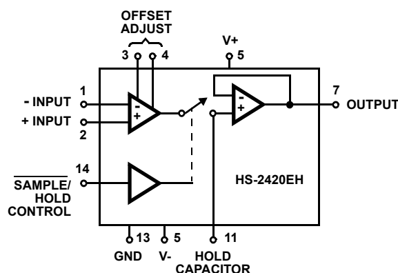
FIGURE 1. FUNCTIONAL DIAGRAM
