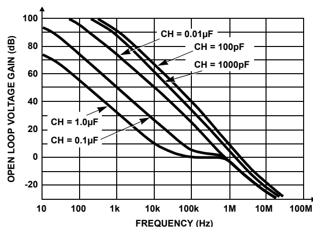
FIGURE 13. OPEN LOOP FREQUENCY RESPONSE
