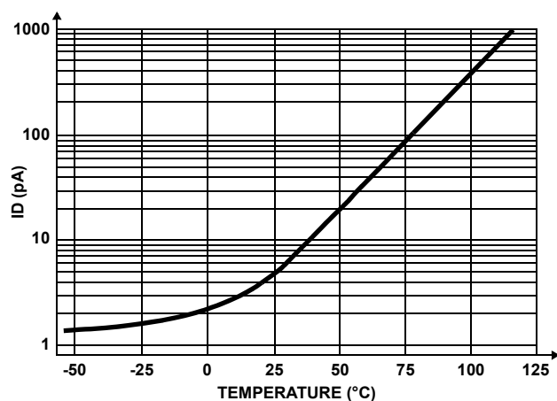
FIGURE 12. DRIFT CURRENT vs TEMPERATURE
