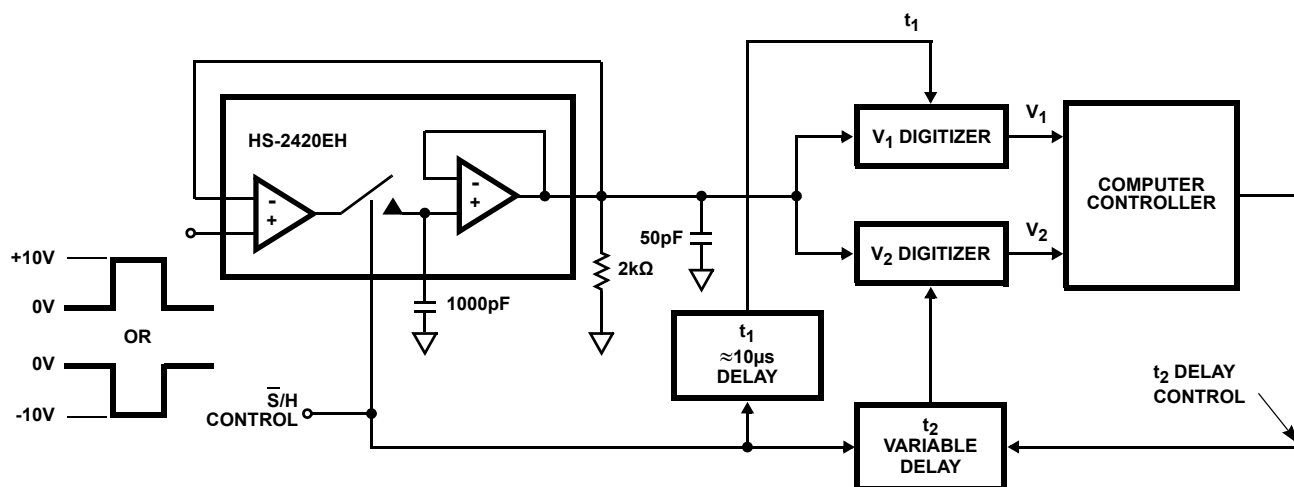
FIGURE 6. BLOCK DIAGRAM FOR ACQUISITION TIME MEASUREMENT
