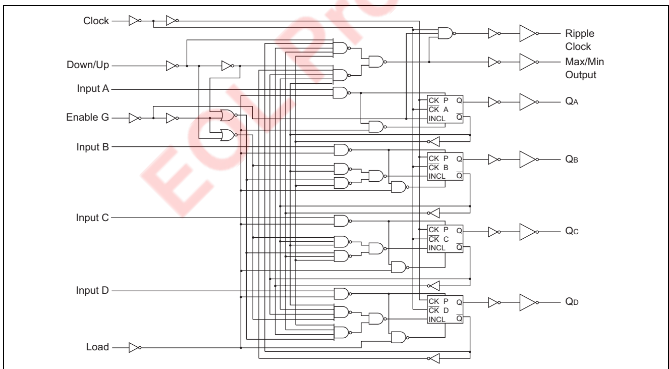
HD74HC191
