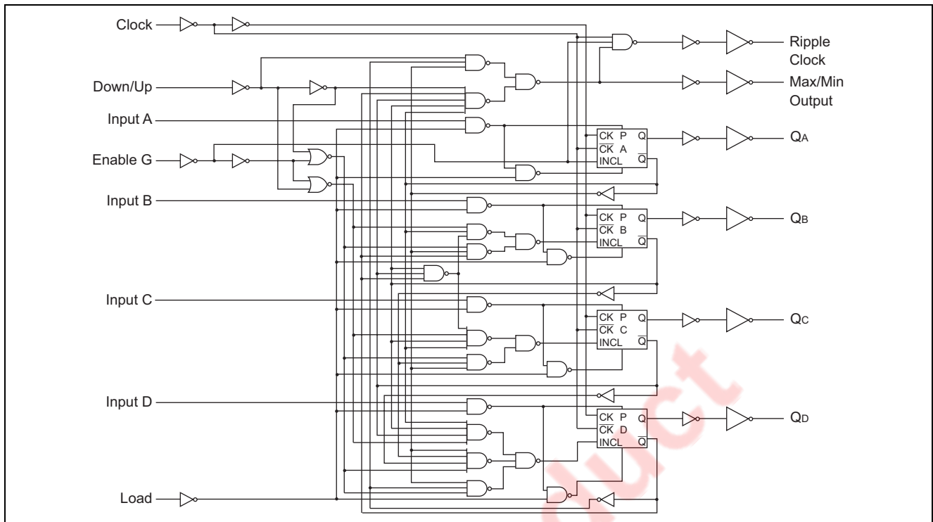
HD74HC191
