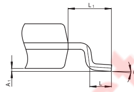
Terminal cross section ( Ni/Pd/Au plating )
