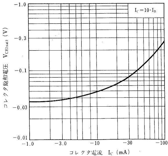
COLLECTOR SATURATION VOLTAGE vs. COLLECTOR CURRENT
