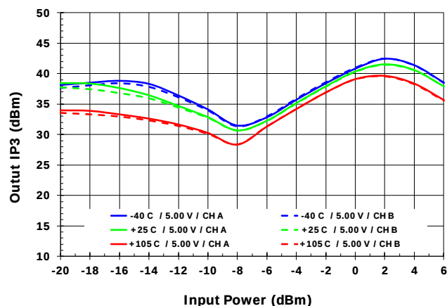
OIP3 vs. Input Power [1100 MHz]
