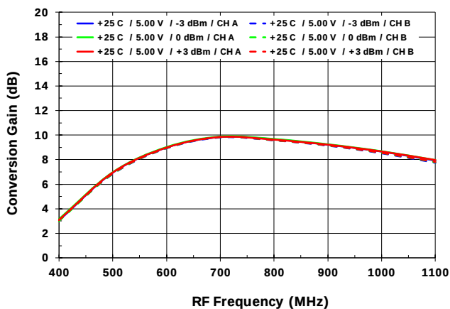
Gain vs. LO Power [ G_{MXR} , HS Injection]
