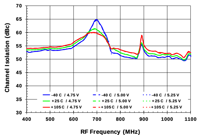
Channel Isolation vs. T_{case} & V_{cc} [ ISO_{B-A} ]
