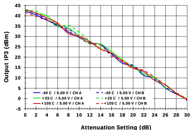
OIP3 vs. Attenuation [1100 MHz]
