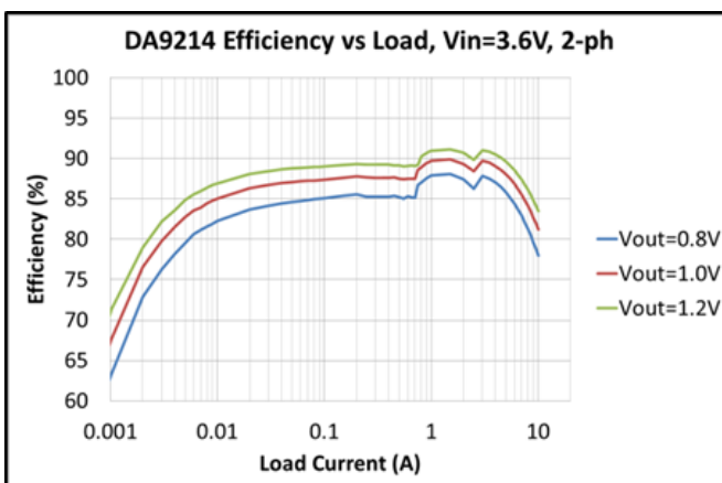
Figure 9. 2 Phase Auto-Mode, 0 A to 10 A
