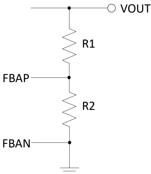
Figure 19. Resistive Divider from VOUT to FBAN
