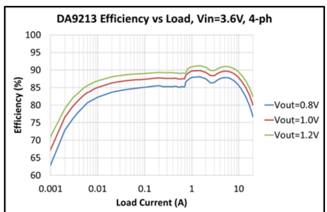
Figure 12. 4 Phase Auto-Mode, 0 A to 20 A
