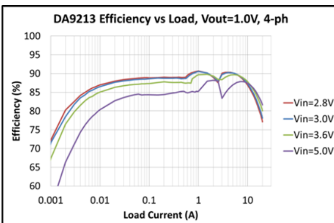
Figure 11. 4 Phase Auto-Mode, 0 A to 20 A (Logarithmic)
