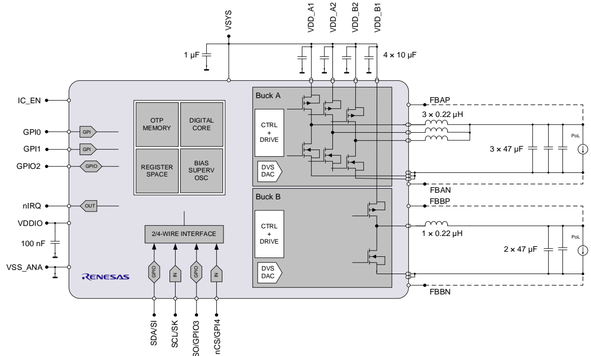
Figure 3. DA9215 System Diagram
