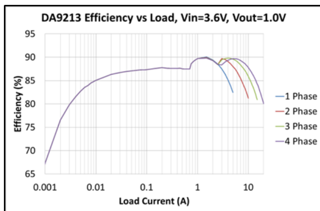
Figure 13. 1, 2, 3, and 4 Phase Modes
