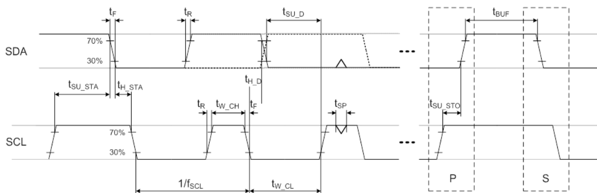
Figure 6. 2-WIRE Bus Timing
