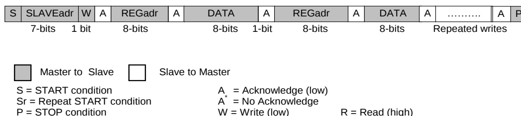
Figure 29. 2-WIRE Repeated Write (SDA Line)
