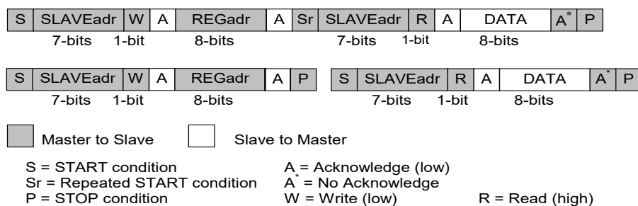
Figure 11. I²C Byte Read (SDA Line) Examples
