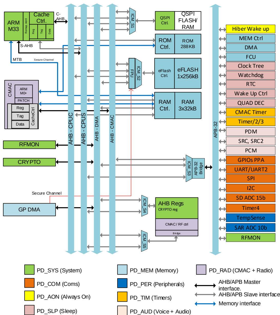
Figure 23. Bus architecture
