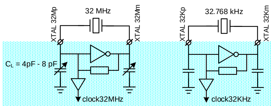
Figure 30. Crystal oscillator circuits
