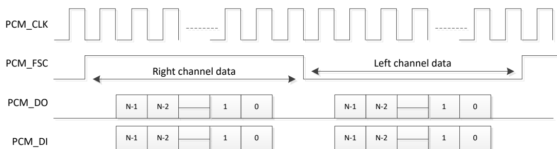
Figure 53. I2S mode
