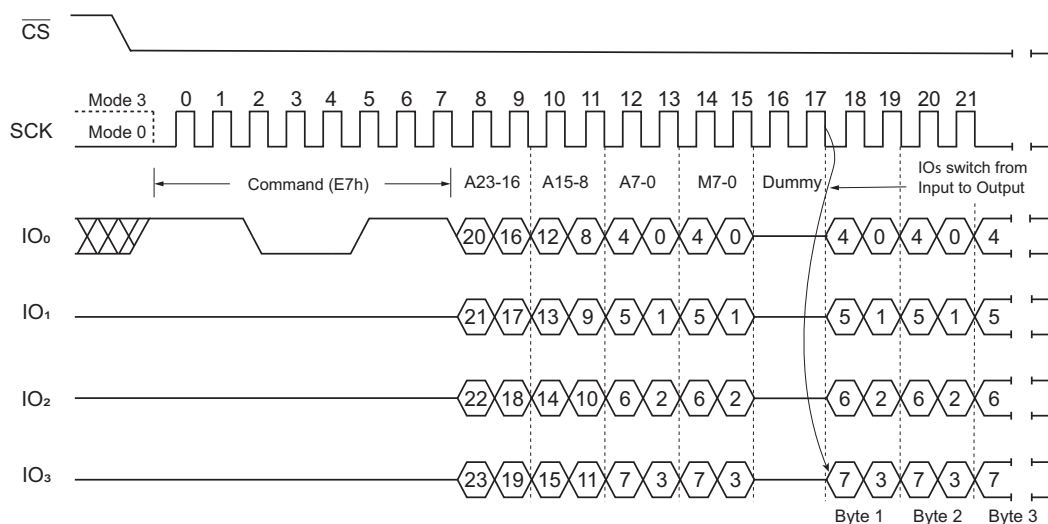
Figure 33. Word Read Quad I/O Command (Initial command or previous set M5-4 \neq 1,0; SPI Mode)
