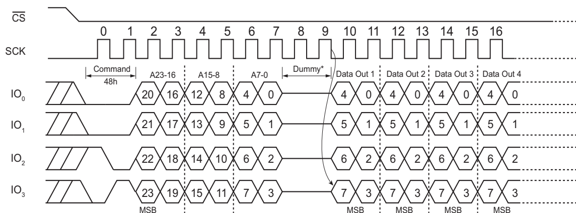
Figure 52. Read Security Register, QPI Mode
