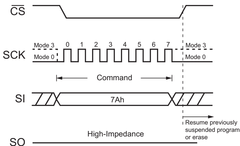
Figure 71. Erase / Program Resume Command (SPI Mode)
