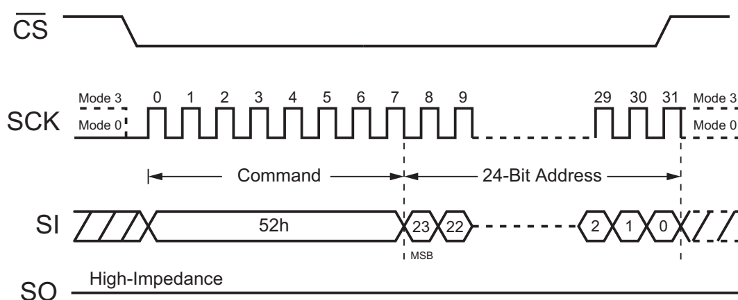
Figure 64. 32-kB Block Erase Command (SPI Mode)
