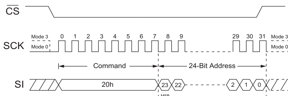
Figure 62. 4-kB Block Erase Command (SPI Mode)
