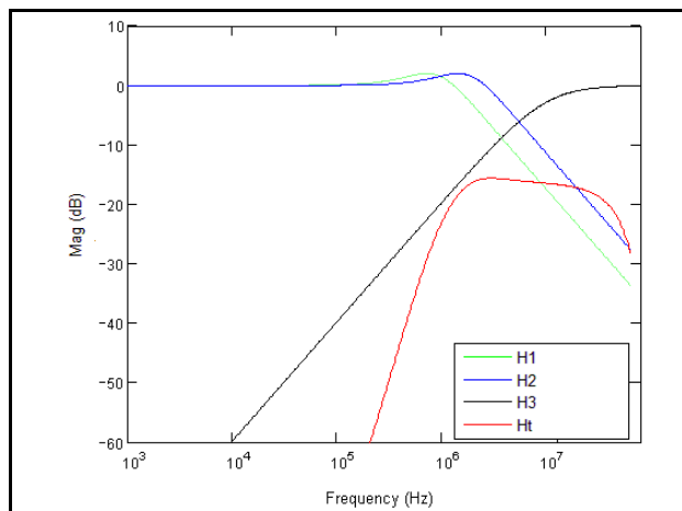
PCI Express Gen 3 Magnitude of Transfer Function
