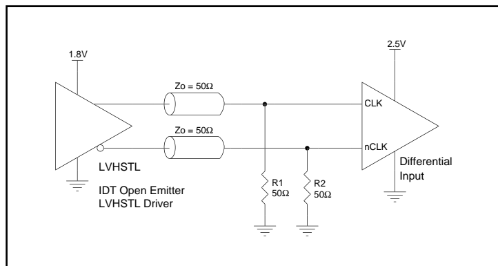
Figure 10A. CLKx/nCLKx Input Driven by an IDT Open Emitter LVHSTL Driver
