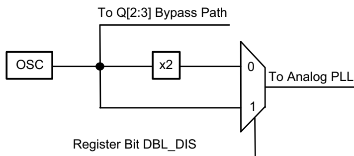
Figure 3. Doubler Block Diagram
