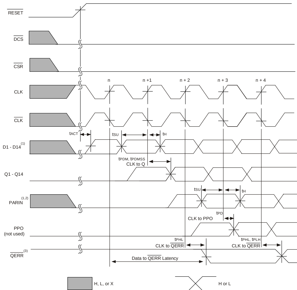
Timing Diagram for the Second IDT74SSTUAE32866A (1:2 Register-B Configuration) Device Used in a Pair; C0 = 1, C1 = 1, \overline{RESET} Switches from L to H
