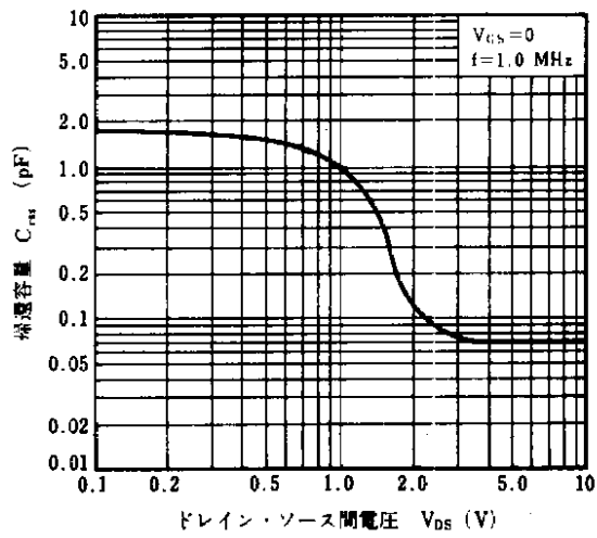
FEEDBACK CAPACITANCE vs. DRAIN TO SOURCE VOLTAGE
