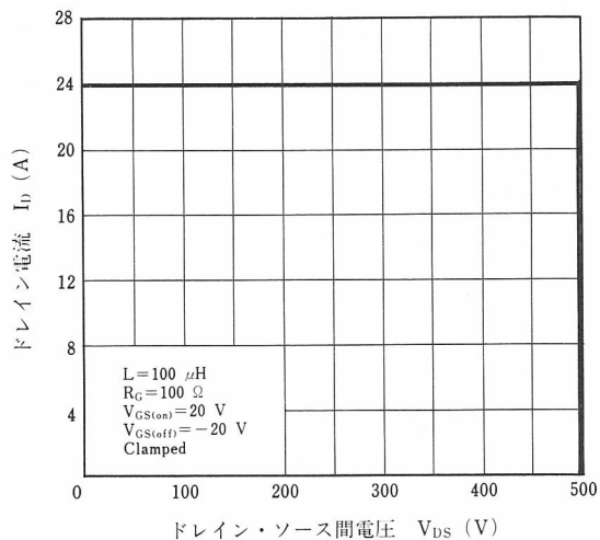
REVERSE BIAS SAFE OPEATING AREA
