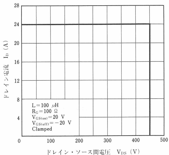
REVERSE BIAS SAFE OPEATING AREA
