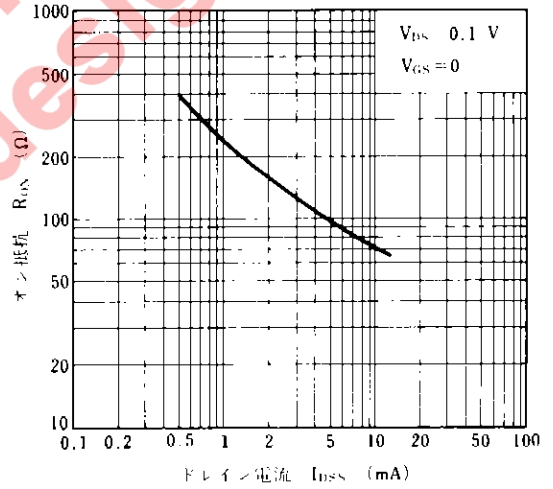
DRAIN TO SOURCE RESISTANCE vs. DRAIN CURRENT
