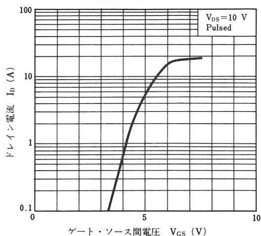
TRANSFER CHARACTERISTIC
