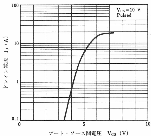
TRANSFER CHARACTERISTIC
