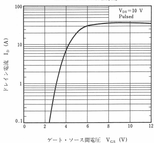
TRANSFER CHARACTERISTIC
