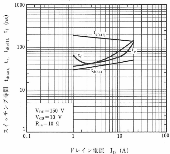
SWITCHING CHARACTERISTICS
