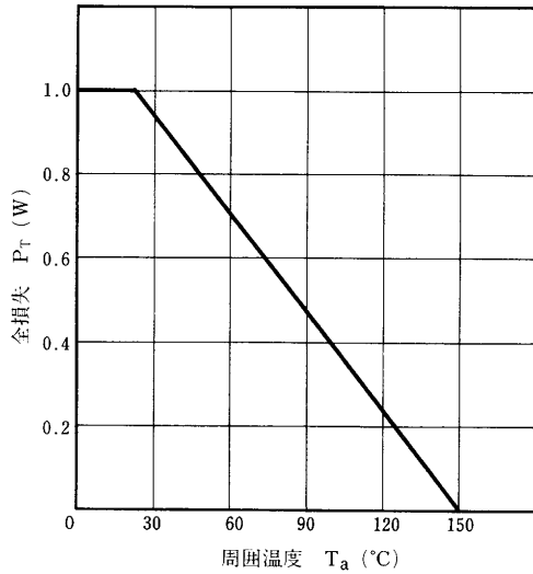
TOTAL POWER DISSIPATION vs. AMBIENT TEMPERATURE
