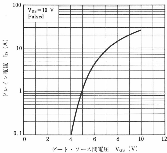
TRANSFER CHARACTERISTIC
