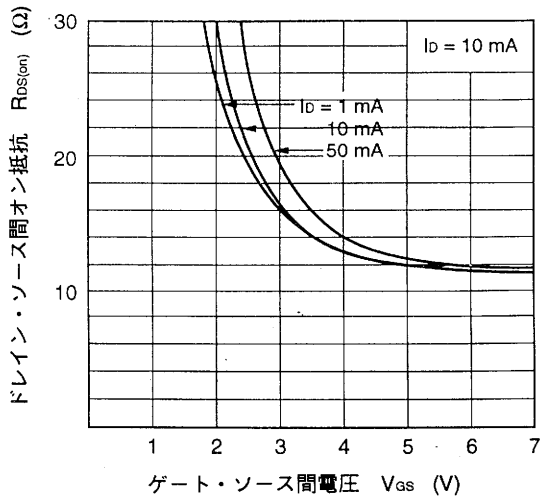
DRAIN TO SOURCE ON-STAGE RESISTANCE vs. GATE TO SOURCE VOLTAGE
