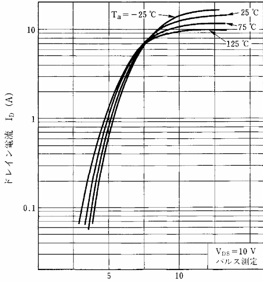
TRANSFER CHARACTERISTICS
