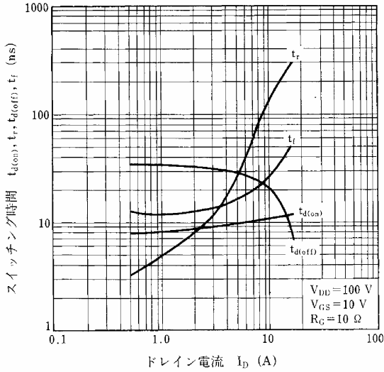
SWITCHING CHARACTERISTICS
