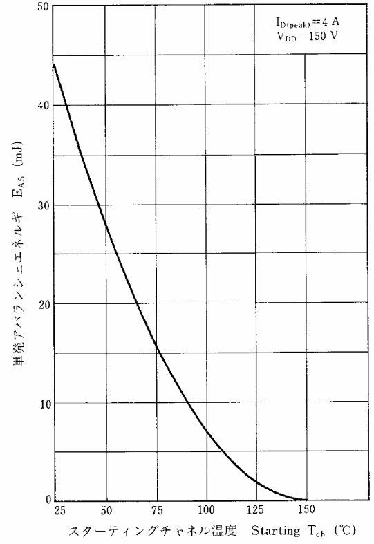
SINGLE AVALANCHE ENERGY vs. STARTING CHANNEL TEMPERATURE
