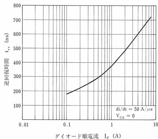
REVERSE RECOVERY TIME vs. REVERSE DRAIN CURRENT
