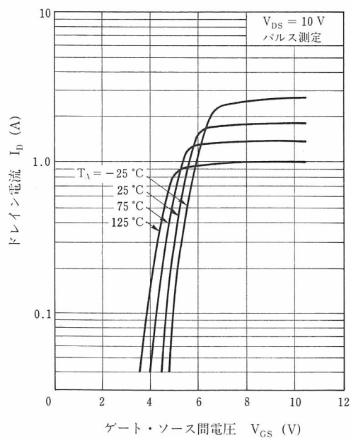
TRANSFER CHARACTERISTICS
