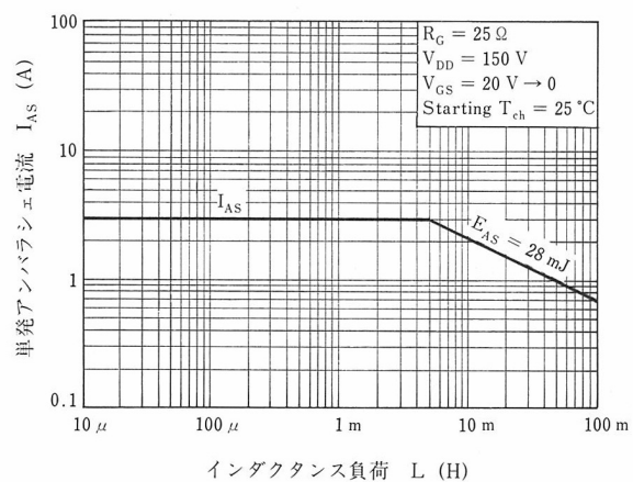
SINGLE AVALANCHE CURRENT vs. INDUCTIVE LOAD
