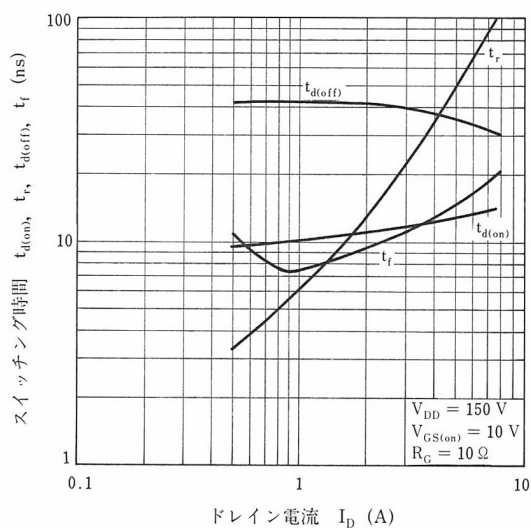
SWITCHING TIME vs. DRAIN CURRENT
