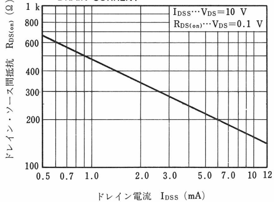
DRAIN TO SOURCE RESISTANCE vs. DRAIN CURRENT
