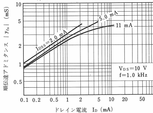
FORWARD TRANSFER ADMITTANCE (yfs) vs. DRAIN CURRENT
