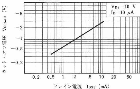
GATE SOURCE CUTOFF VOLTAGE vs. ZERO-GATE VOLTAGE DRAIN CURRENT
