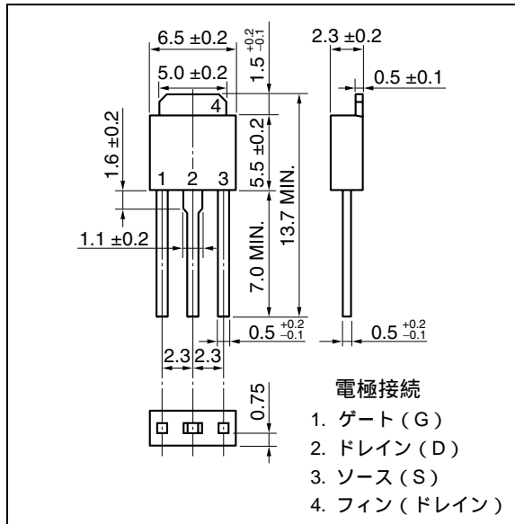
1) TO-251 (MP-3)
