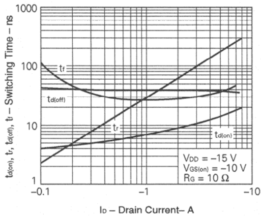
SWITCHING CHARACTERISTICS
