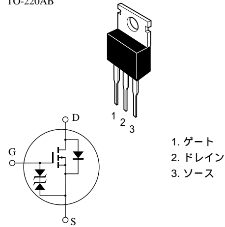
TO-220AB
