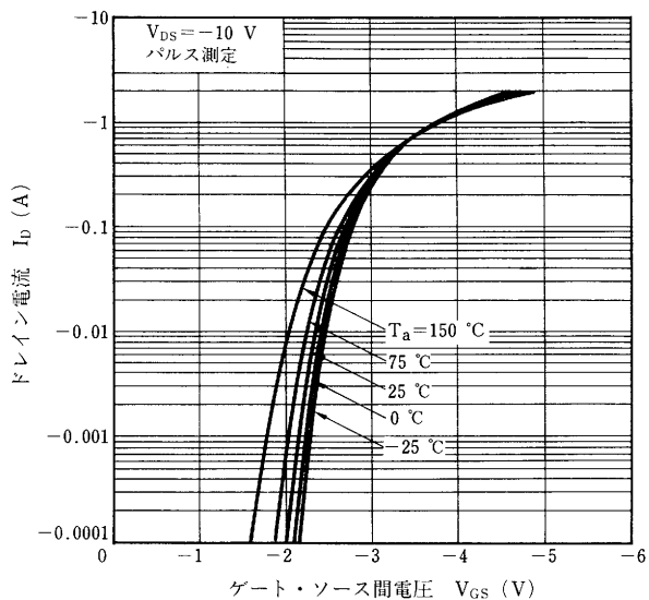
TRANSFER CHARACTERISTICS
