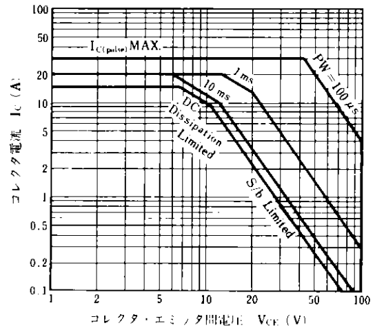
SAFE OPERATING AREAS
