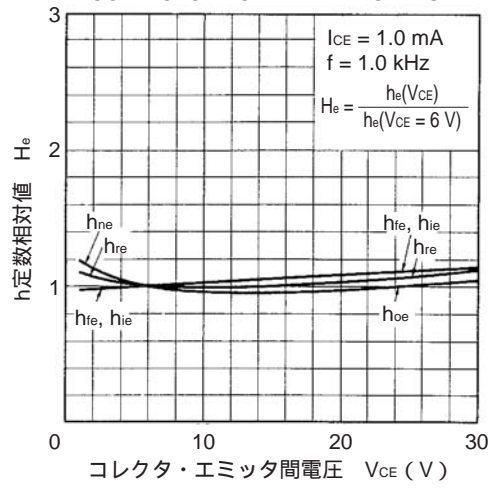
NORMALIZED h-PARAMETER vs. COLLECTOR TO EMITTER VOLTAGE
