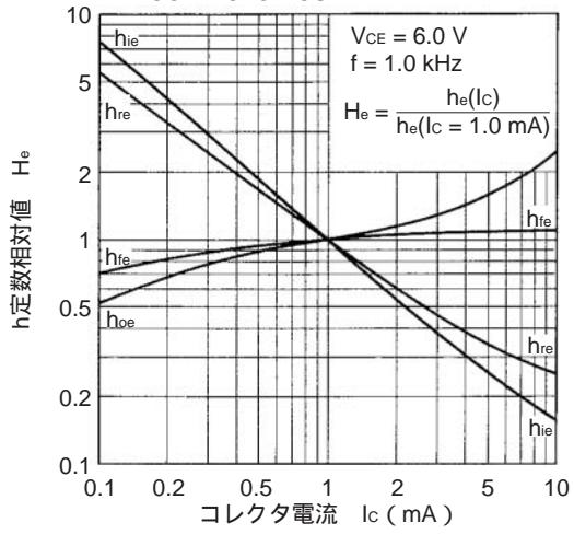
NORMALIZED h-PARAMETER vs. COLLECTOR CURRENT
