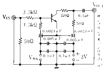
T_{on}, T_{off} TEST CIRCUIT
