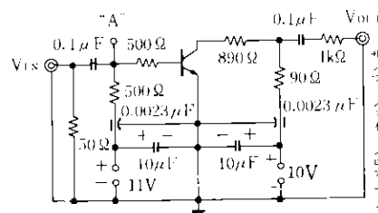
T_{sta} TEST CIRCUIT
