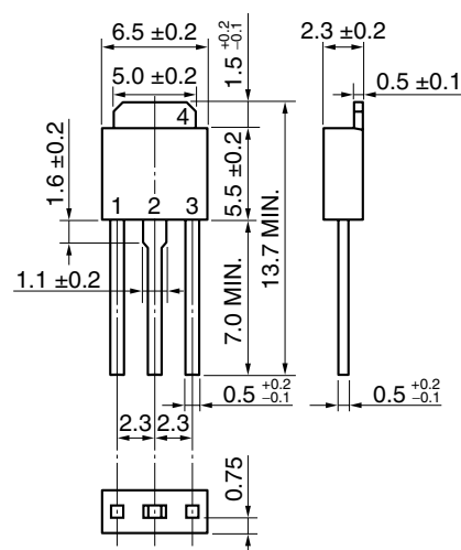
TO-251 (MP-3)
