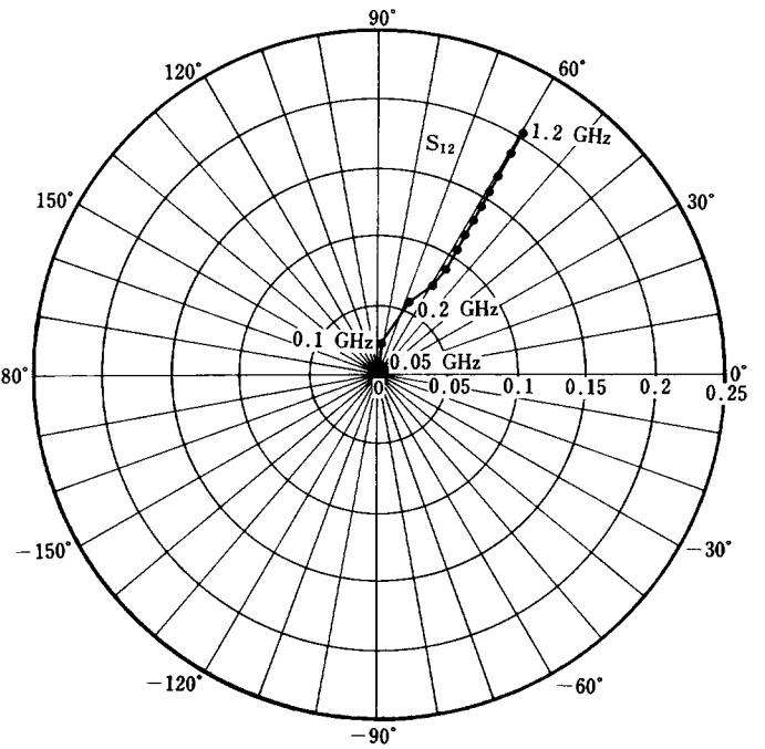
S_{12e} -FREQUENCY CONDITION V_{CE}=10\text{ V}, I_C=5\text{ mA}
