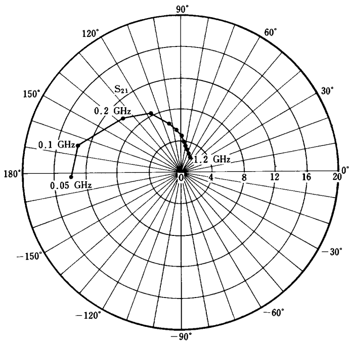
S_{21e} -FREQUENCY CONDITION V_{CE}=10\text{ V}, I_C=5\text{ mA}
