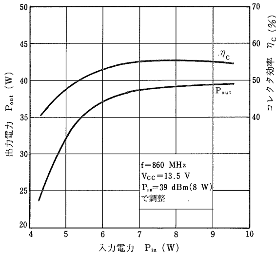
OUTPUT POWER AND COLLECTOR EFFICIENCY vs. INPUT POWER CURVE
