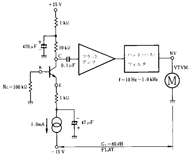
V_{CE} \approx 5V, I_C = 1.0mA, R_C = 100k\Omega, G_r = 80dB, FLAT (f = 10Hz \sim 1.0kHz)
