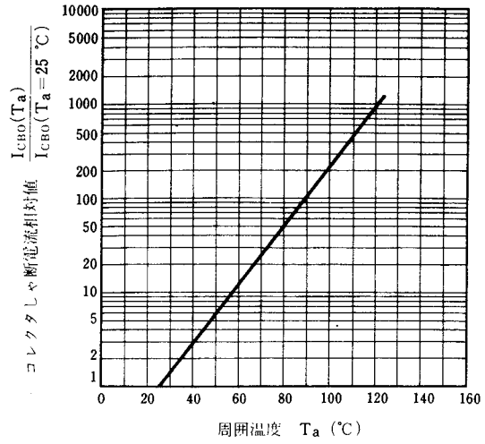
NORMALIZED COLLECTOR CUTOFF CURRENT vs. AMBIENT TEMPERATURE
