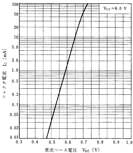
COLLECTOR CURRENT vs. BASE TO EMITTER VOLTAGE
