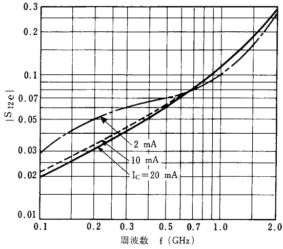
REVERSE TRANSFER COEFFICIENT vs. FREQUENCY
