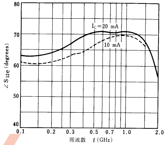
REVERSE TRANSFER COEFFICIENT vs. FREQUENCY
