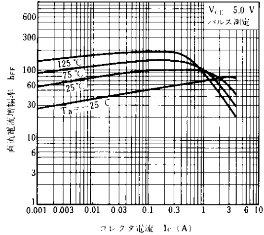
2SD743, 2SD743A DC CURRENT GAIN vs. COLLECTOR CURRENT
