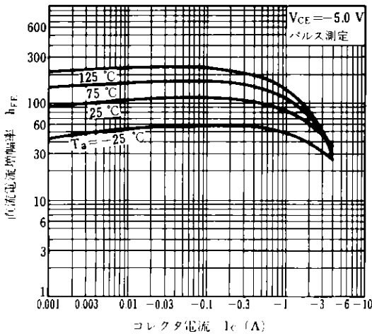
2SB703, 2SB703A DC CURRENT GAIN vs. COLLECTOR CURRENT
