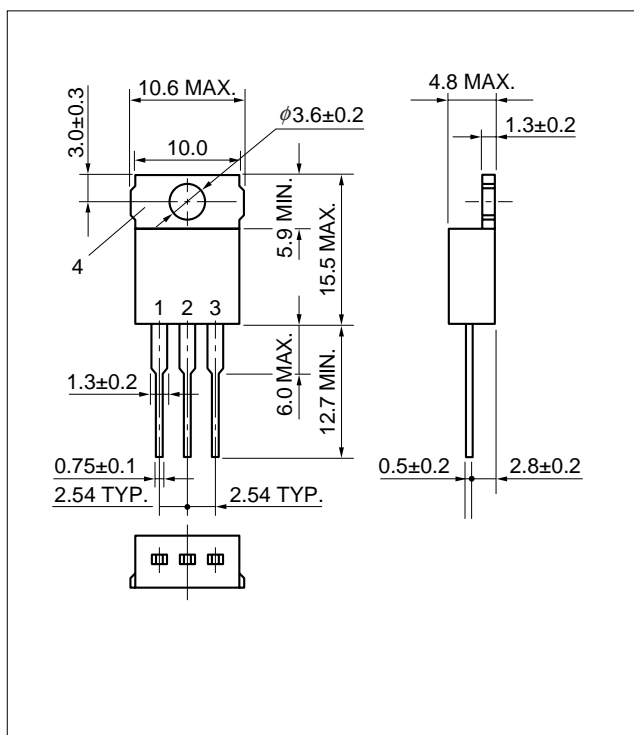
TO-220AB (MP-25)
