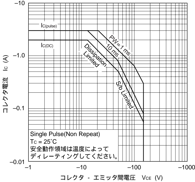
FORWARD BIAS SAFE OPERATING AREA
