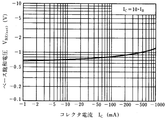
BASE SATURATION VOLTAGE vs. COLLECTOR CURRENT
