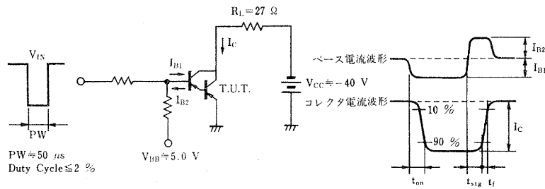
SWITCHING TIME ( t_{on} , t_{stg} , t_f ) TEST CIRCUIT
