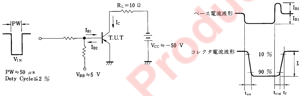
SWITCHING TIME ( t_{on} , t_{str} , t_f ) TEST CIRCUIT
