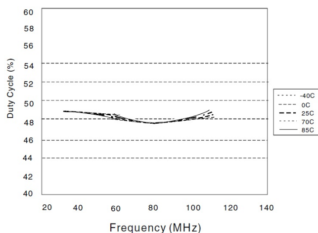
Figure 19. Duty Cycle vs Frequency (10pF loads over temperature – 3.3V)
