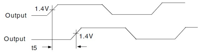
Figure 4. Output-to-Output Skew
