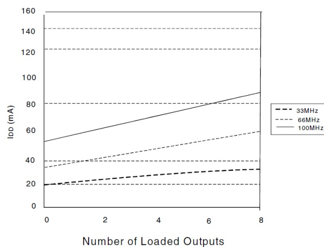
Figure 21. IDD vs Number of Loaded Outputs (for 10pF loads over frequency – 3.3V, 25°C)
