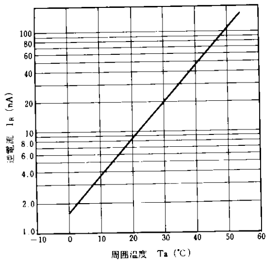
REVERSE CURRENT vs. AMBIENT TEMPERATURE
