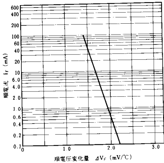
FORWARD CURRENT vs. TEMPERATURE COEFFICIENT
