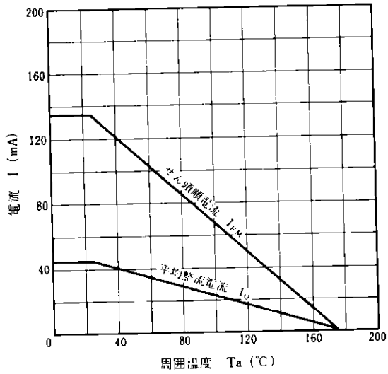
AVERAGE RECTIFIED CURRENT AND PEAK FORWARD CURRENT vs. AMBIENT TEMPERATURE
