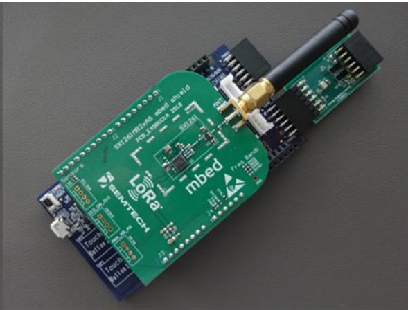
RL78/G23-128p Fast Prototyping Board + SX1261/SX1262 Shield + HS3001 Humidity Sensor
