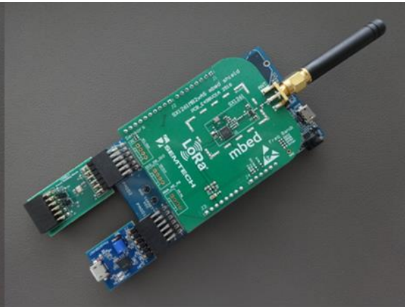
RL78/G14 Fast Prototyping Board + SX1261/SX1262 Shield + HS3001 Humidity Sensor
