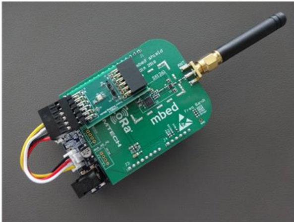
RL78/G23-64p Fast Prototyping Board + SX1261/SX1262 Shield + HS3001 Humidity Sensor
