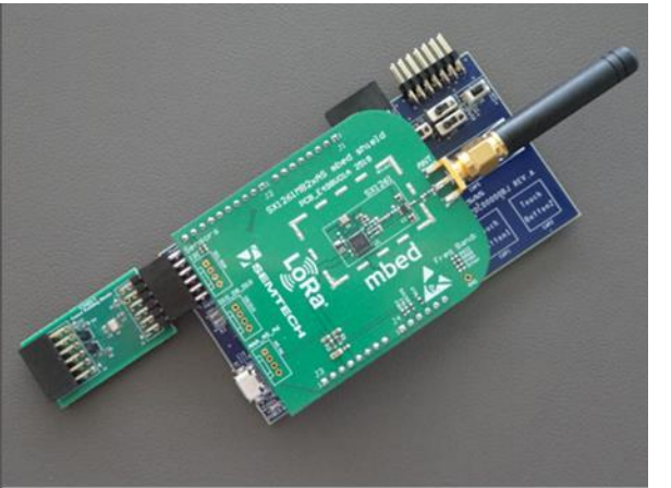
RL78/G22 Fast Prototyping Board + SX1261/SX1262 Shield + HS3001 Humidity Sensor
