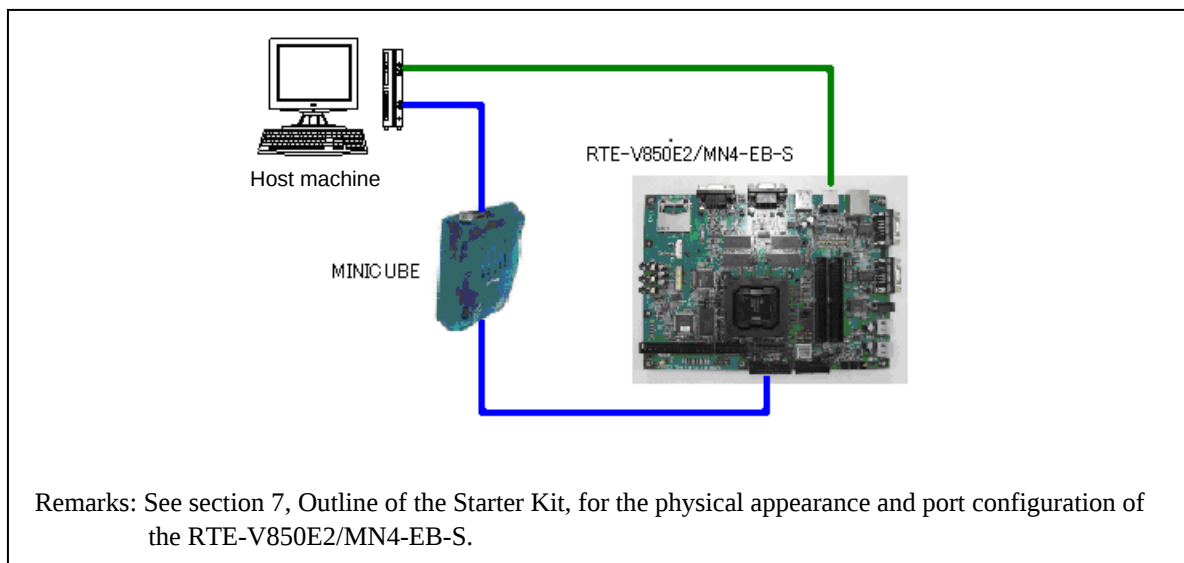
Figure 5.1 System Configuration of the Development Environment
