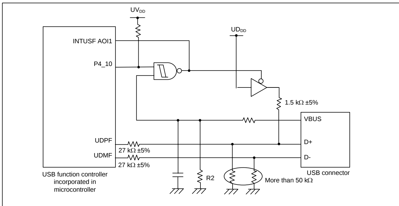
Figure 4.11 USB Function Controller Configuration Example
