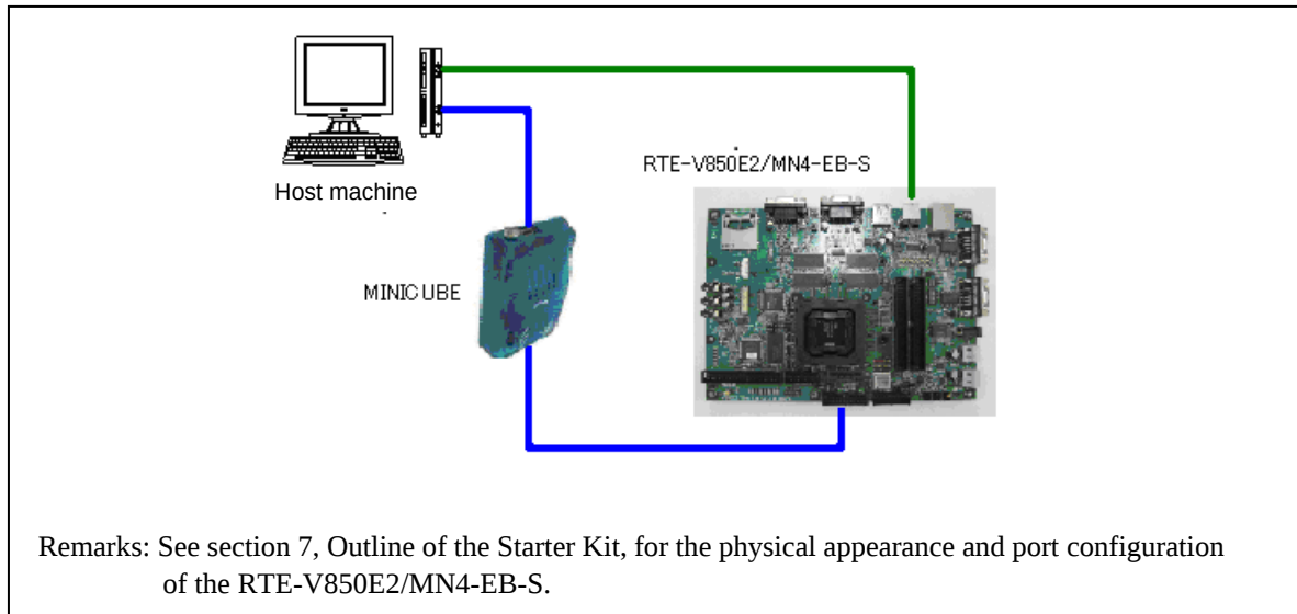
Figure 5.9 Connecting the RTE-V850E2/MN4-EB-S
