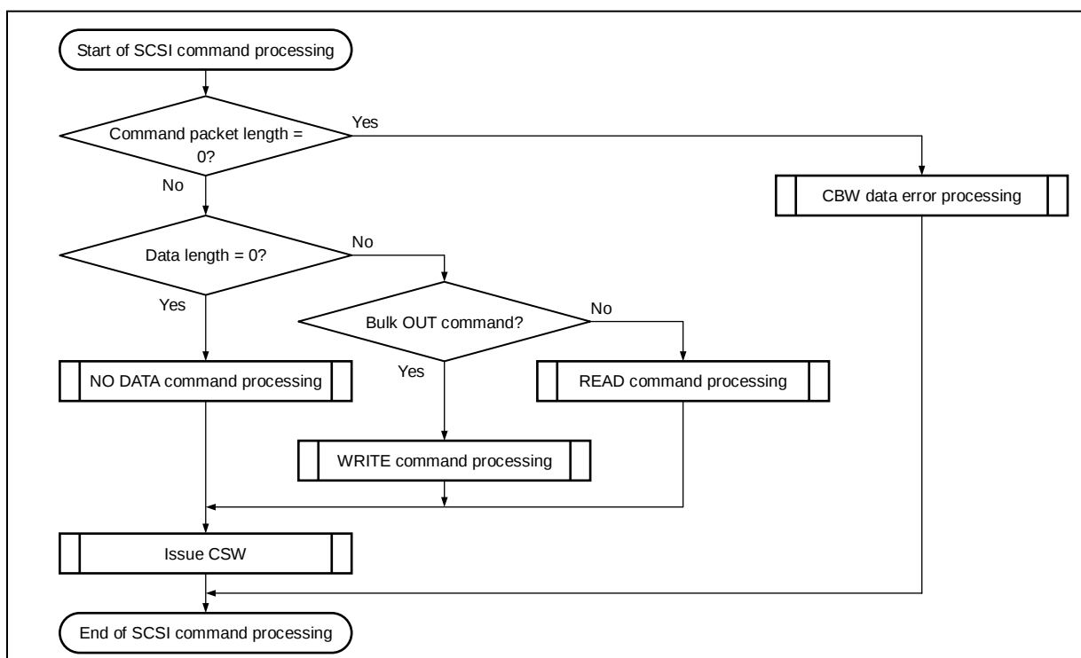
Figure 4.15 SCSI Command Processing Flow
