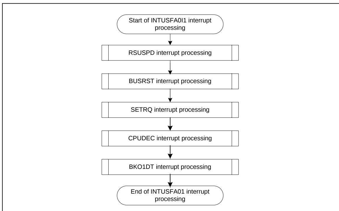
Figure 4.12 INTUSFA0I1 Interrupt Handler Processing Flow
