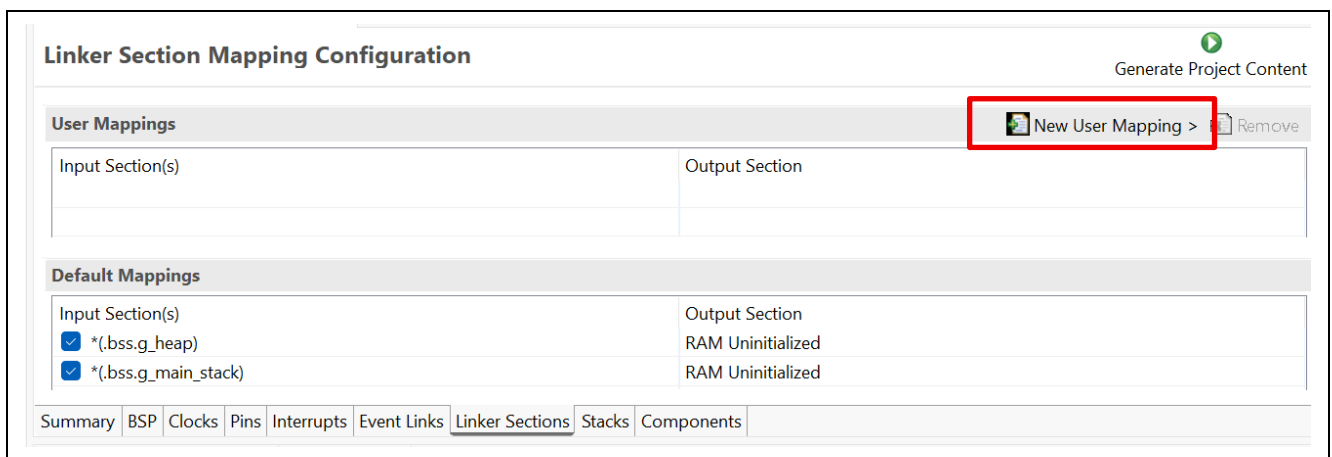
Figure 14. Customize the Memory Region Assignment using the RA Smart Configurator
