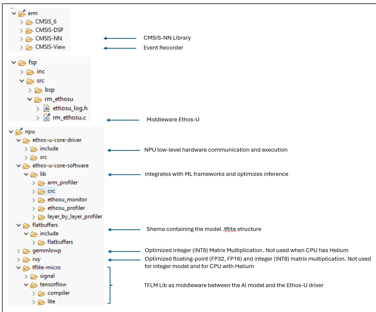
Figure 10. FSP Generated Code for NPU Usage
