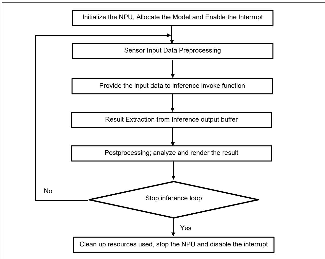
Figure 13. Typical AI Inference Flow
