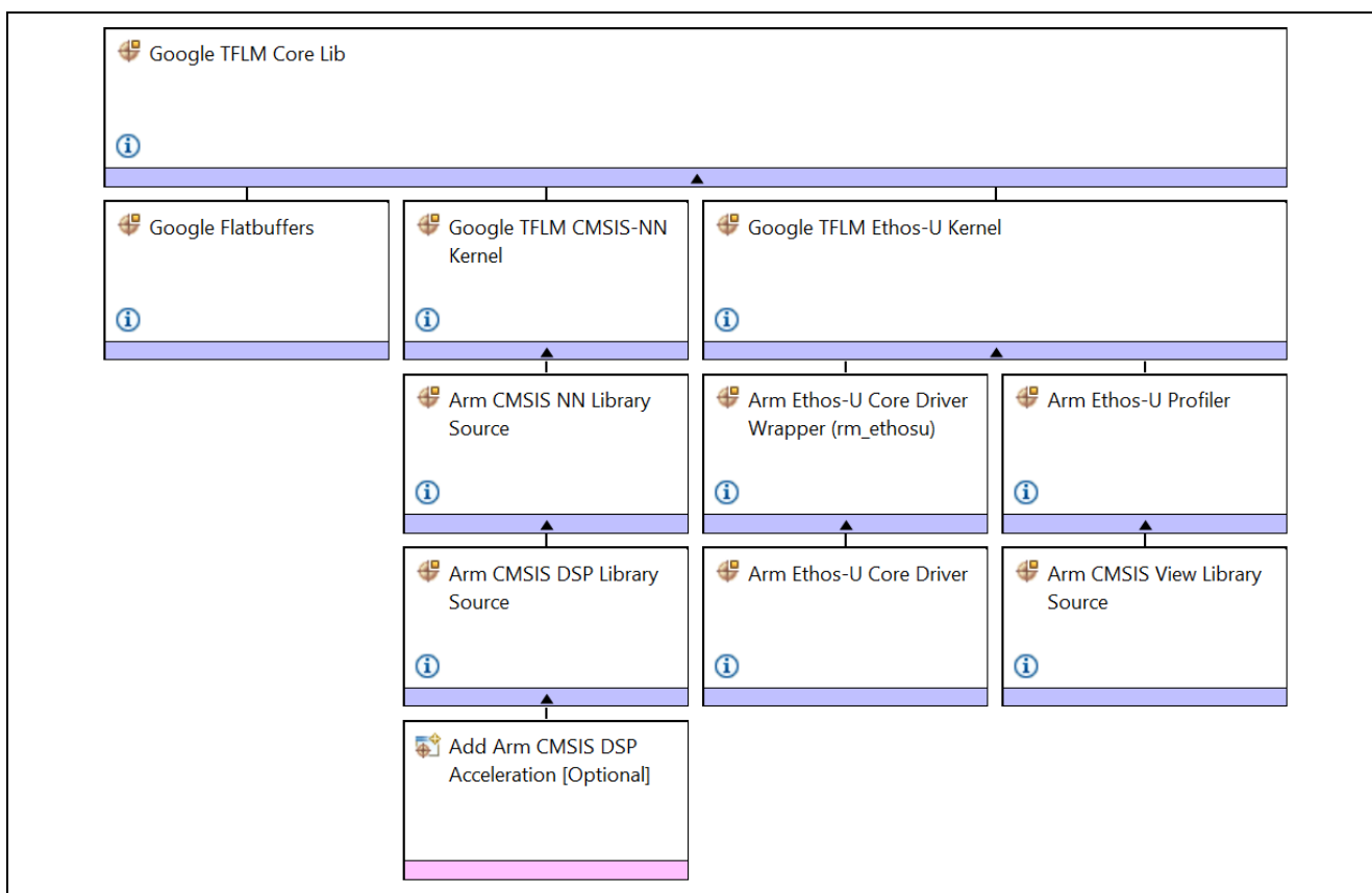
Figure 9. TFLM Core Library for Ethos-U
